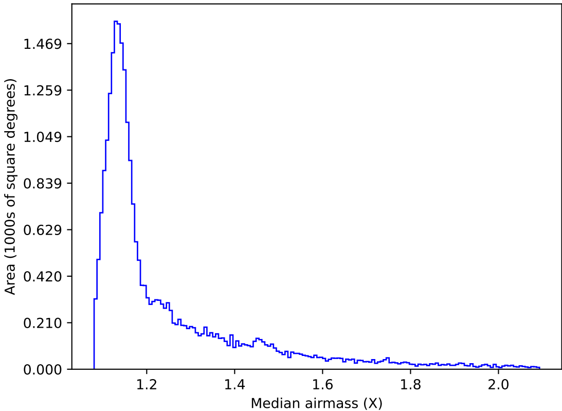
too_elab_r8_d2_griz_v3.4_10yrs All sky i band: Median airmass
