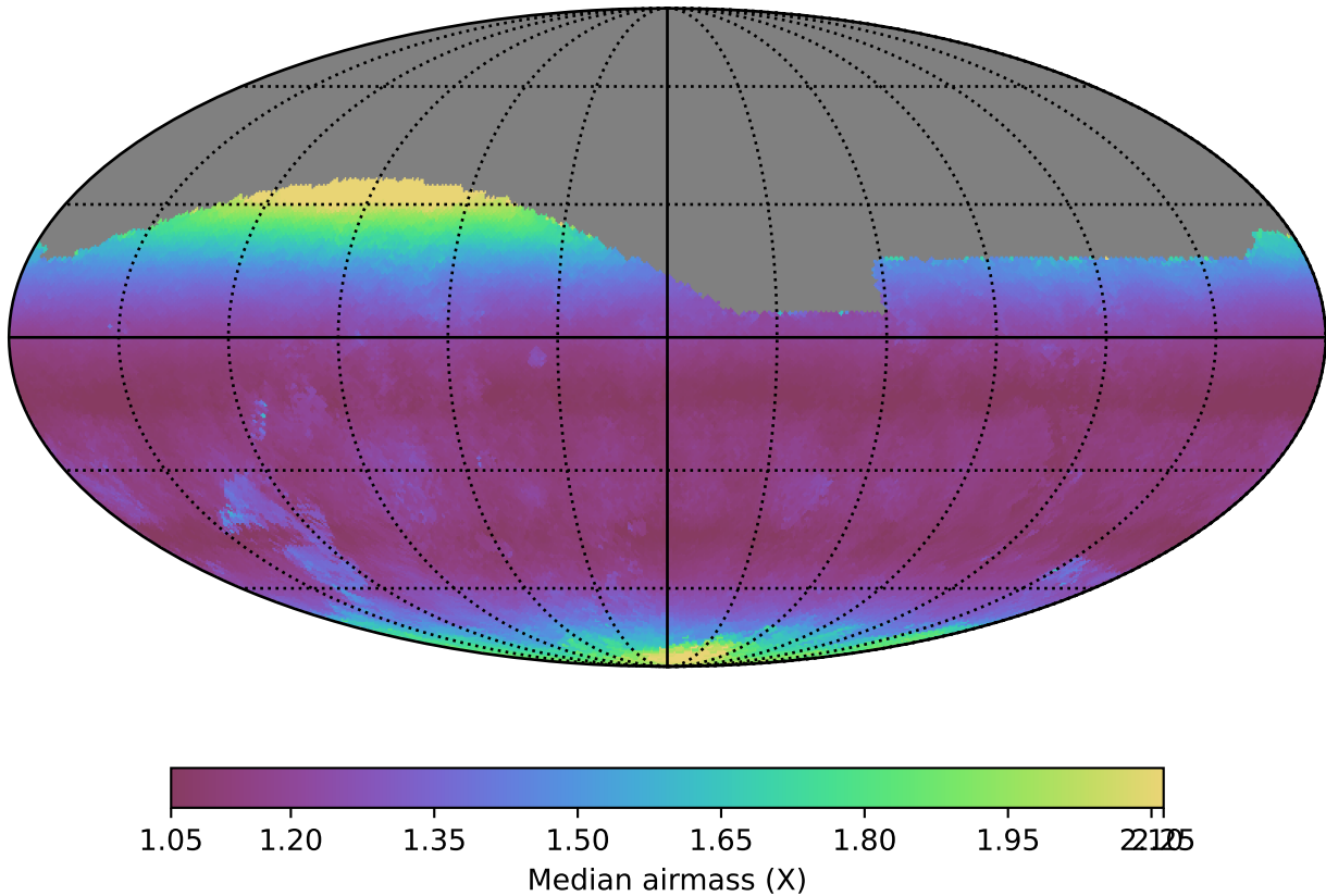
too_elab_r8_d2_griz_v3.4_10yrs All sky g band: Median airmass
