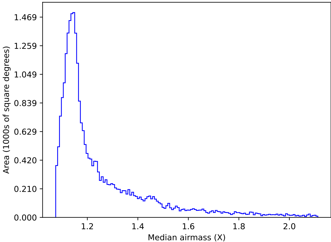
too_elab_r8_d2_griz_v3.4_10yrs All sky g band: Median airmass
