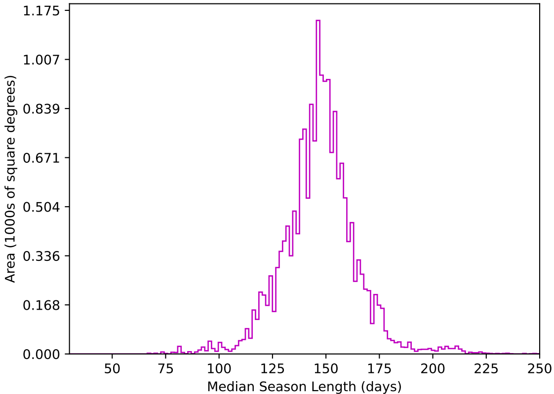
too_elab_r8_d2_griz_v3.4_10yrs WFD z band: Median Season Length
