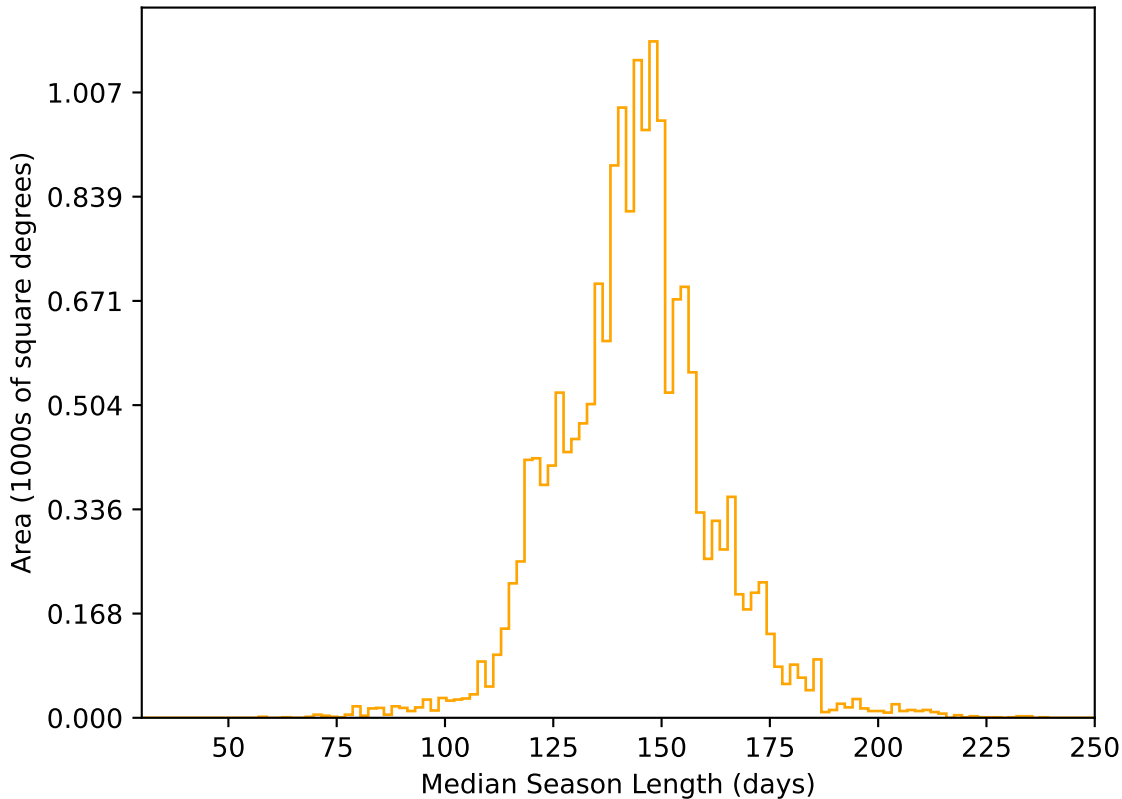
too_elab_r8_d2_griz_v3.4_10yrs WFD r band: Median Season Length
