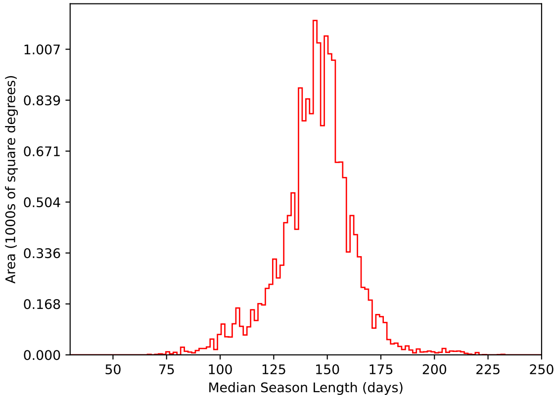
too_elab_r8_d2_griz_v3.4_10yrs WFD i band: Median Season Length
