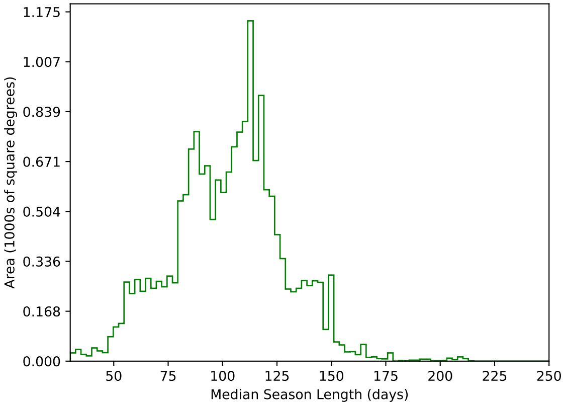
too_elab_r8_d2_griz_v3.4_10yrs WFD g band: Median Season Length
