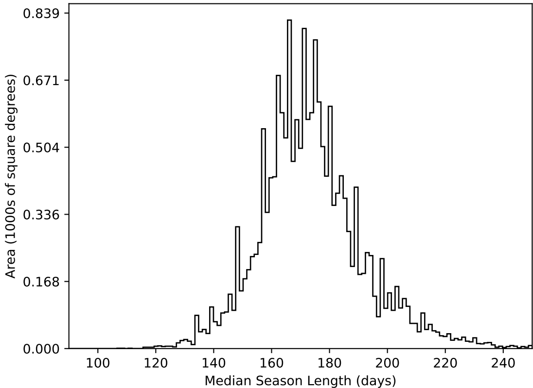
too_elab_r8_d2_griz_v3.4_10yrs WFD all bands: Median Season Length
