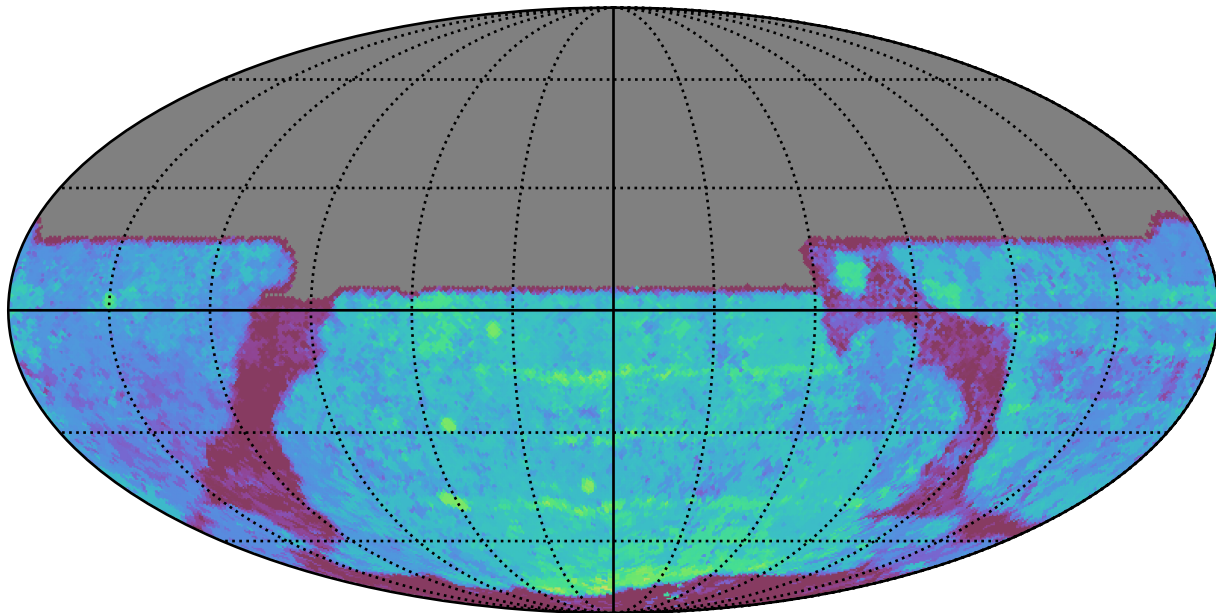
too_elab_r8_d2_griz_v3.4_10yrs All sky y band: Median Season Length
