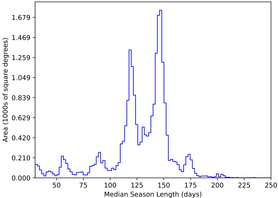
too_elab_r8_d2_griz_v3.4_10yrs All sky y band: Median Season Length
