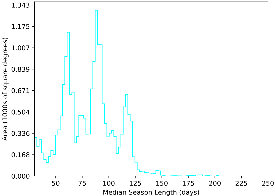
too_elab_r8_d2_griz_v3.4_10yrs All sky u band: Median Season Length
