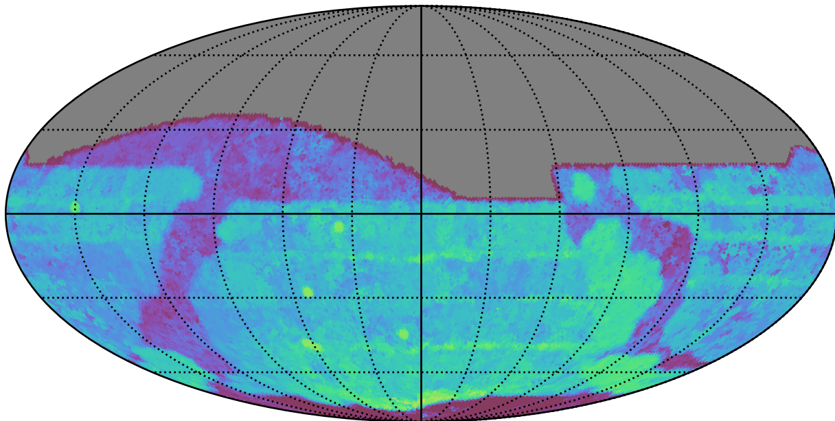
too_elab_r8_d2_griz_v3.4_10yrs All sky r band: Median Season Length
