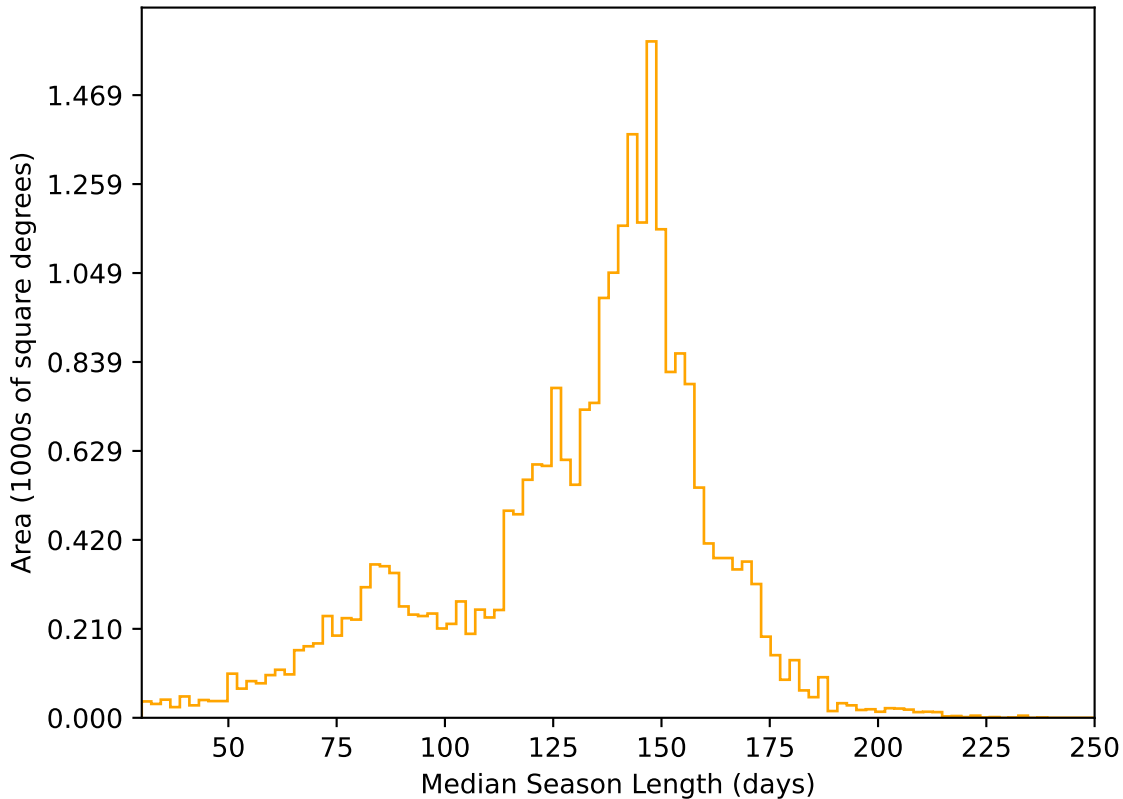
too_elab_r8_d2_griz_v3.4_10yrs All sky r band: Median Season Length
