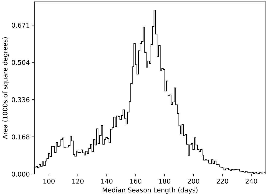
too_elab_r8_d2_griz_v3.4_10yrs All sky all bands: Median Season Length
