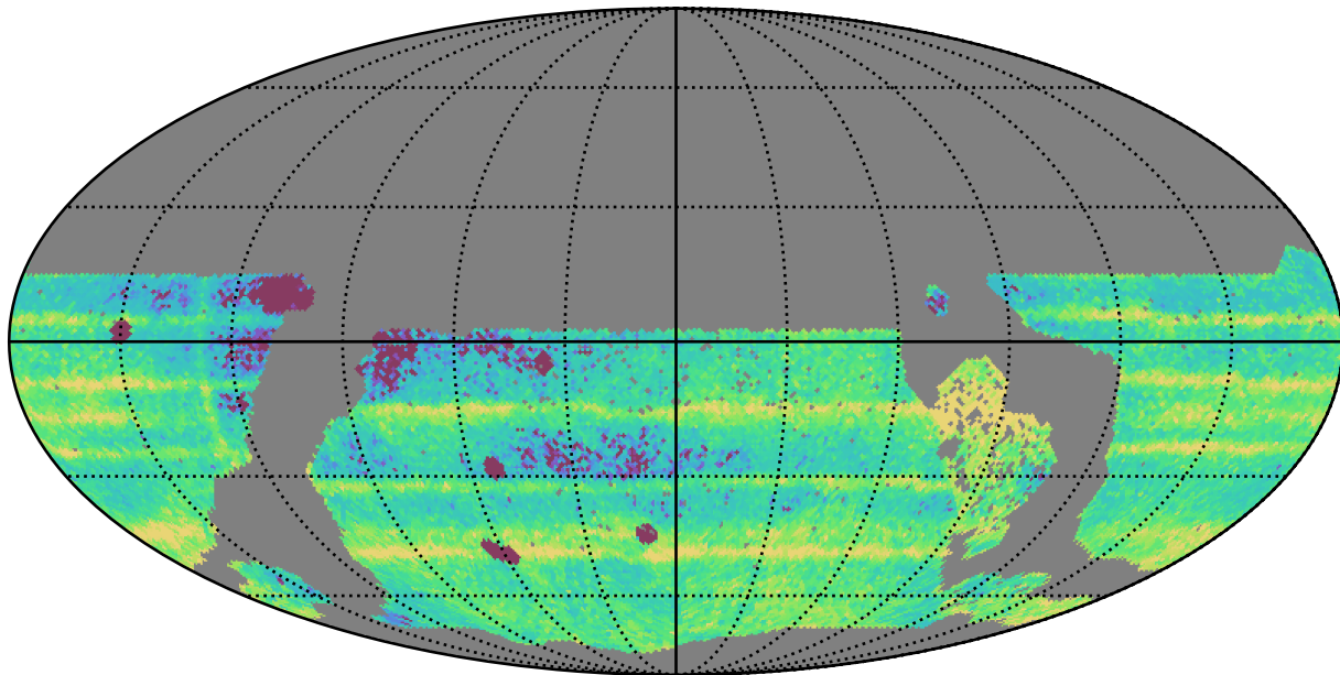
too_elab_r8_d2_griz_v3.4_10yrs WFD: Median Intra-Night Gap
