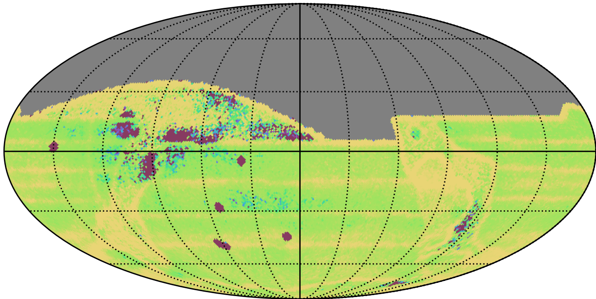
too_elab_r8_d2_griz_v3.4_10yrs All sky: Median Intra-Night Gap
