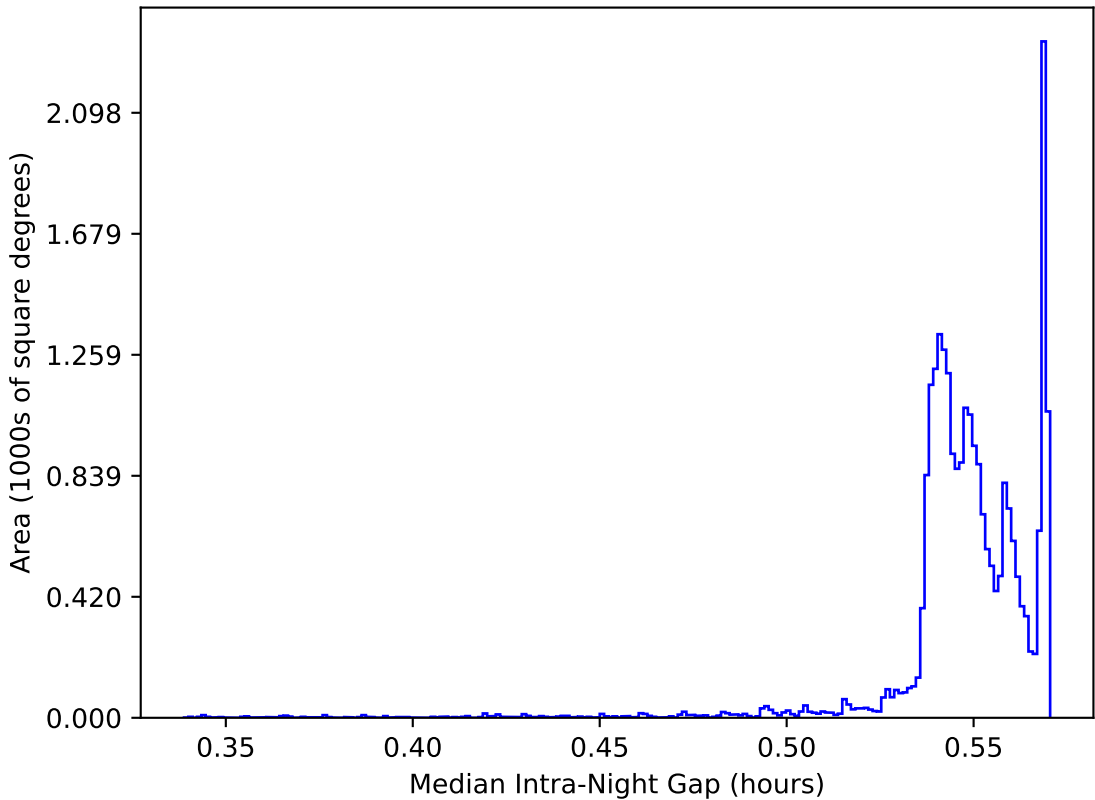
too_elab_r8_d2_griz_v3.4_10yrs All sky: Median Intra-Night Gap
