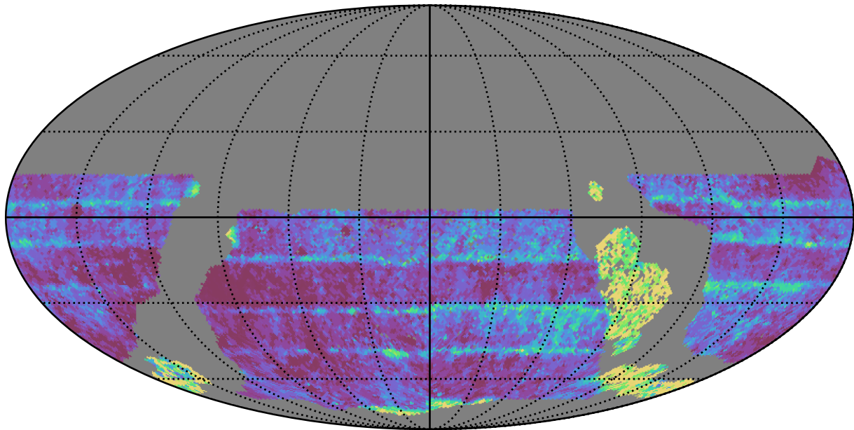
too_elab_r8_d2_griz_v3.4_10yrs WFD z band: Median Inter-Night Gap
