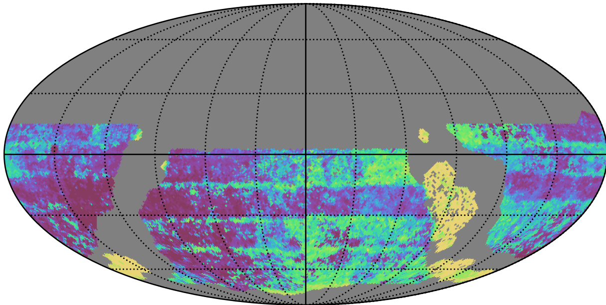
too_elab_r8_d2_griz_v3.4_10yrs WFD y band: Median Inter-Night Gap
