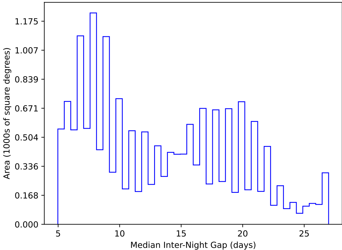
too_elab_r8_d2_griz_v3.4_10yrs WFD y band: Median Inter-Night Gap
