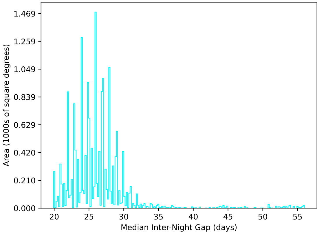
too_elab_r8_d2_griz_v3.4_10yrs WFD u band: Median Inter-Night Gap
