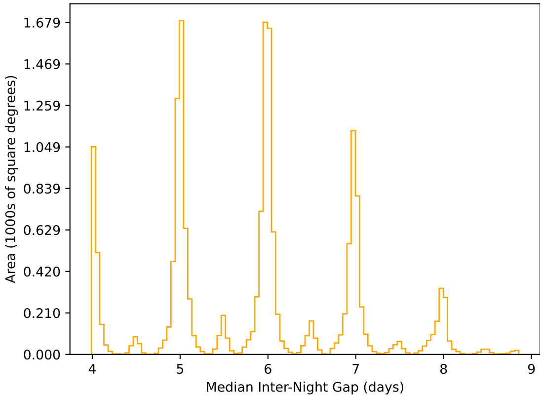
too_elab_r8_d2_griz_v3.4_10yrs WFD r band: Median Inter-Night Gap
