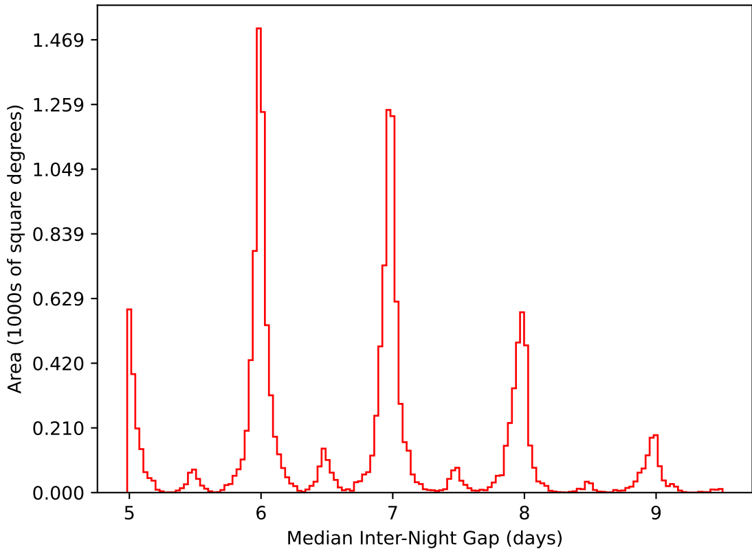
too_elab_r8_d2_griz_v3.4_10yrs WFD i band: Median Inter-Night Gap
