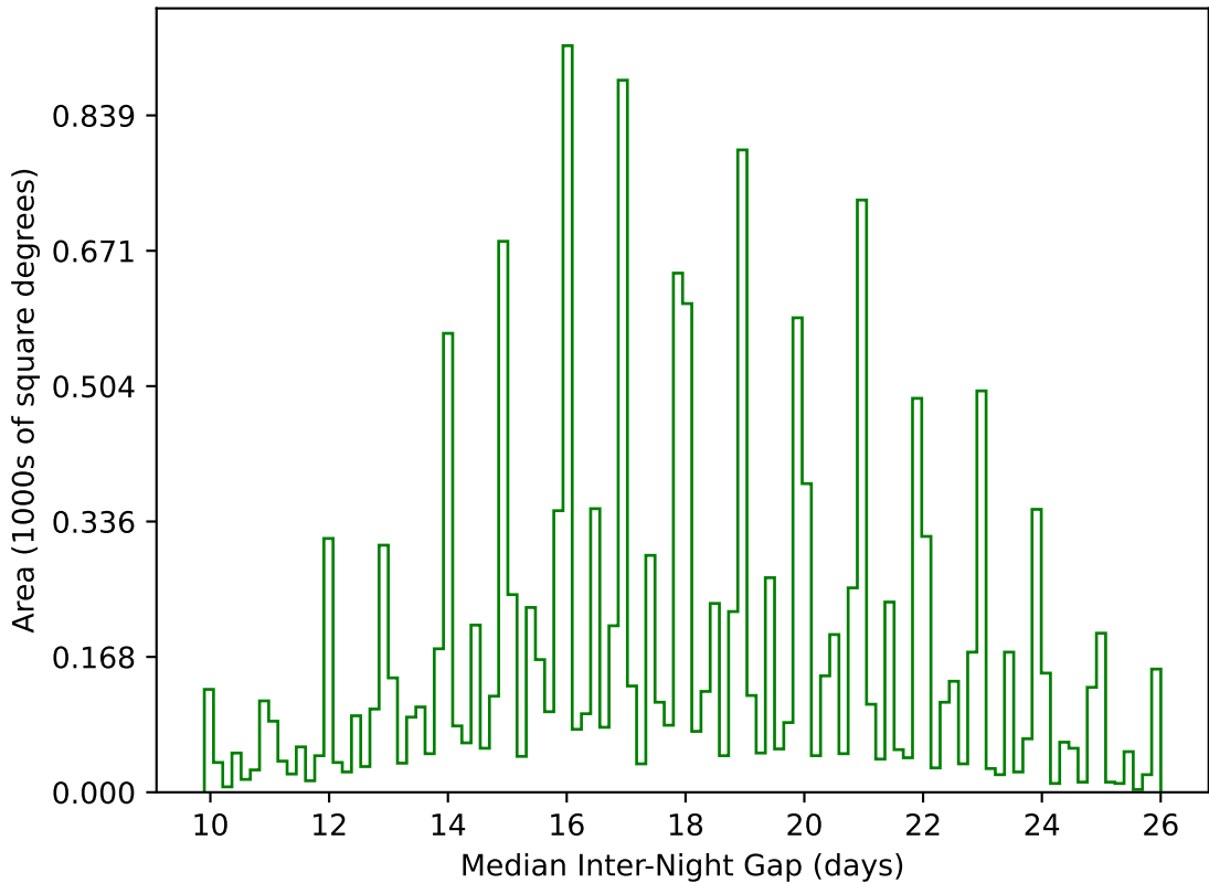
too_elab_r8_d2_griz_v3.4_10yrs WFD g band: Median Inter-Night Gap
