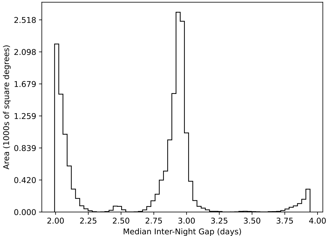
too_elab_r8_d2_griz_v3.4_10yrs WFD all bands: Median Inter-Night Gap
