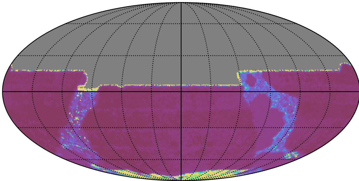
too_elab_r8_d2_griz_v3.4_10yrs All sky y band: Median Inter-Night Gap
