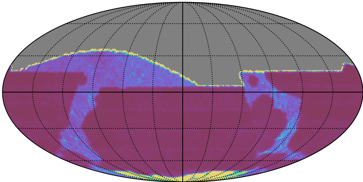
too_elab_r8_d2_griz_v3.4_10yrs All sky r band: Median Inter-Night Gap
