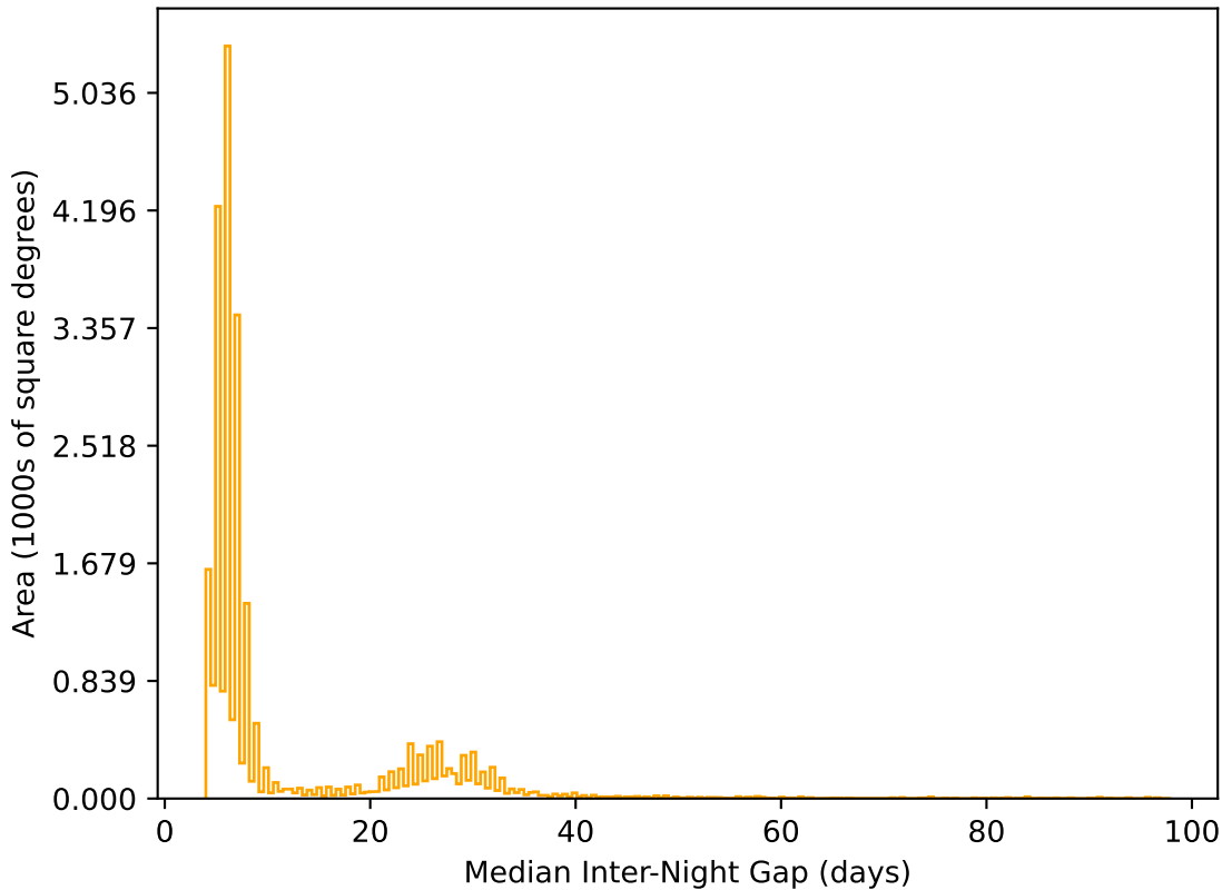
too_elab_r8_d2_griz_v3.4_10yrs All sky r band: Median Inter-Night Gap
