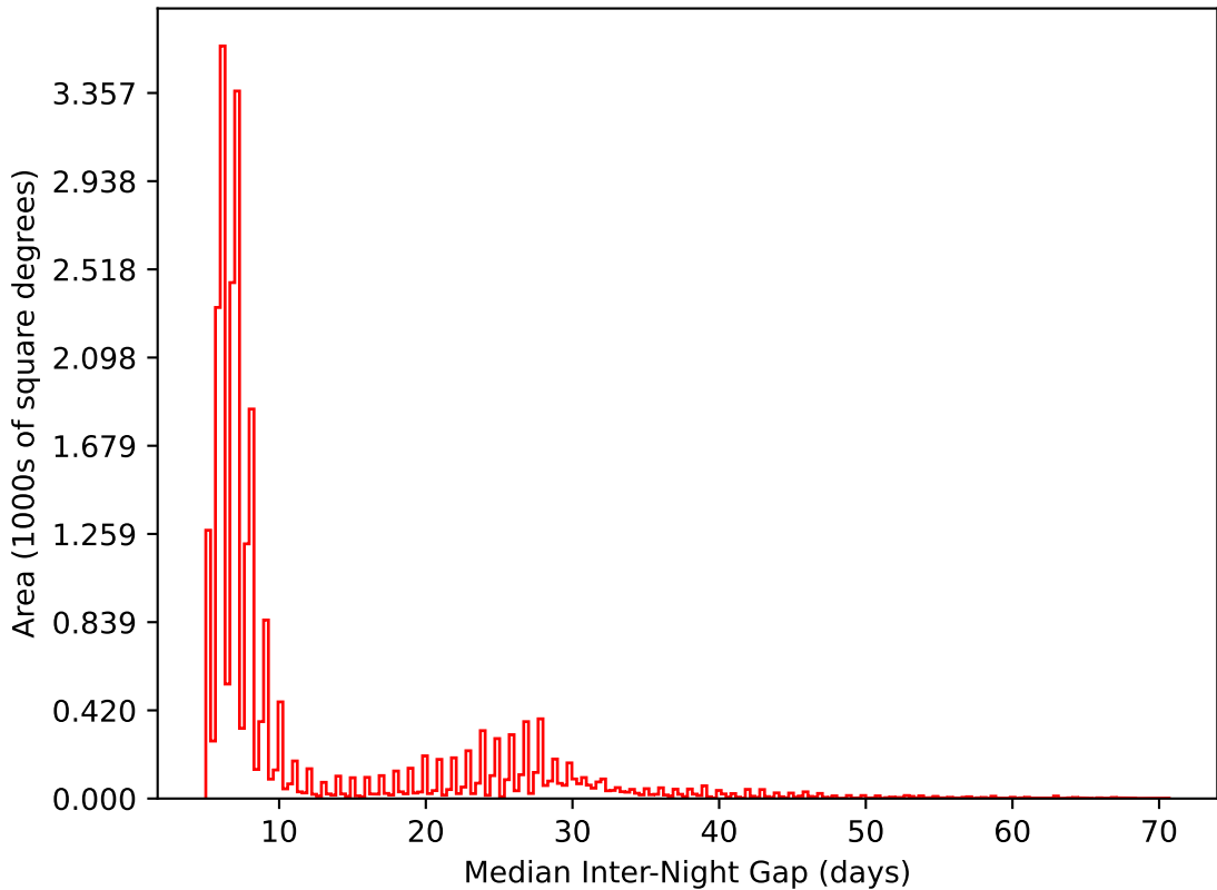
too_elab_r8_d2_griz_v3.4_10yrs All sky i band: Median Inter-Night Gap
