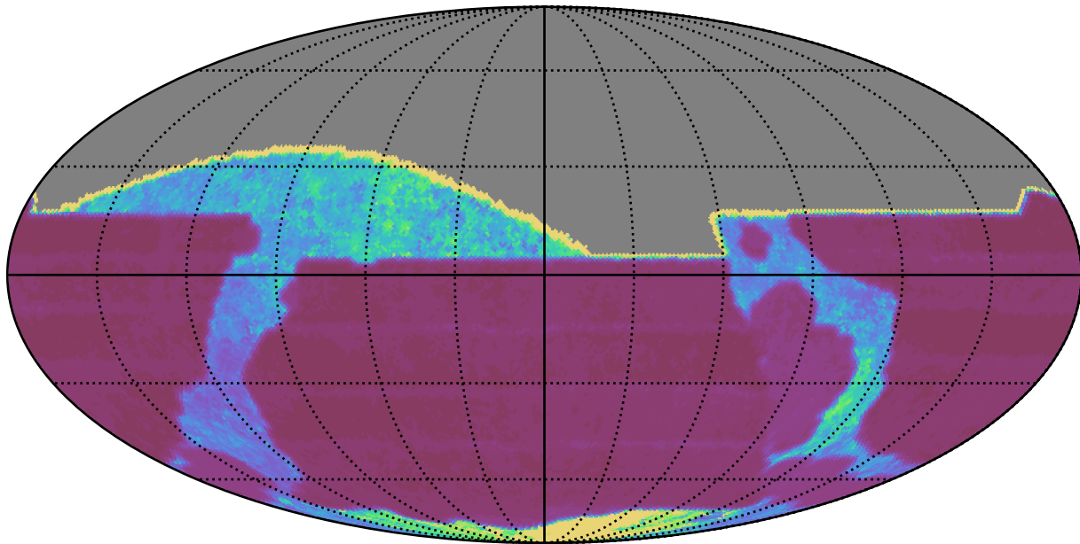
too_elab_r8_d2_griz_v3.4_10yrs All sky all bands: Median Inter-Night Gap
