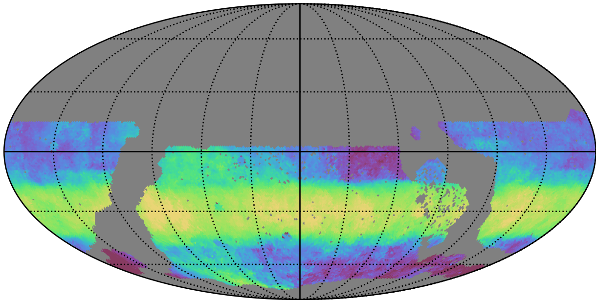
too_elab_r8_d2_griz_v3.4_10yrs WFD z band: Median HA
