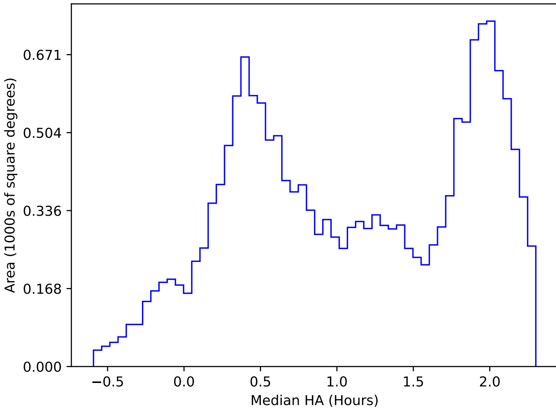
too_elab_r8_d2_griz_v3.4_10yrs WFD z band: Median HA
