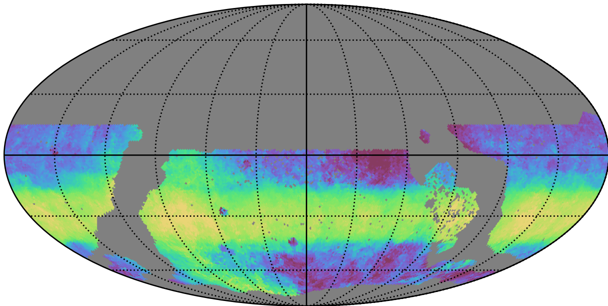
too_elab_r8_d2_griz_v3.4_10yrs WFD y band: Median HA
