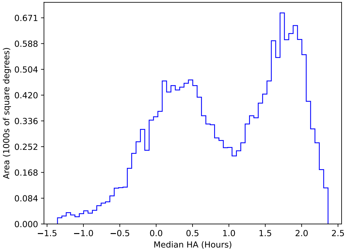
too_elab_r8_d2_griz_v3.4_10yrs WFD u band: Median HA
