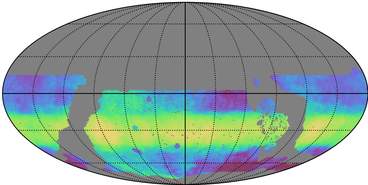
too_elab_r8_d2_griz_v3.4_10yrs WFD i band: Median HA
