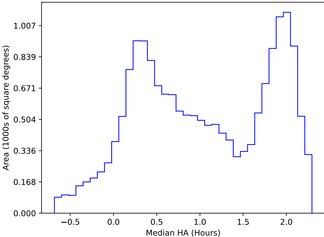
too_elab_r8_d2_griz_v3.4_10yrs WFD i band: Median HA
