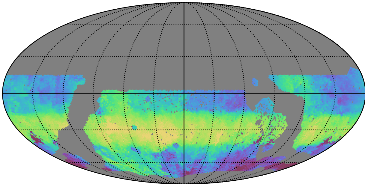
too_elab_r8_d2_griz_v3.4_10yrs WFD g band: Median HA
