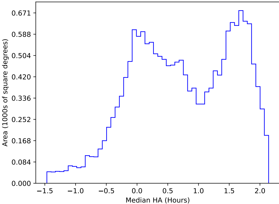
too_elab_r8_d2_griz_v3.4_10yrs WFD g band: Median HA
