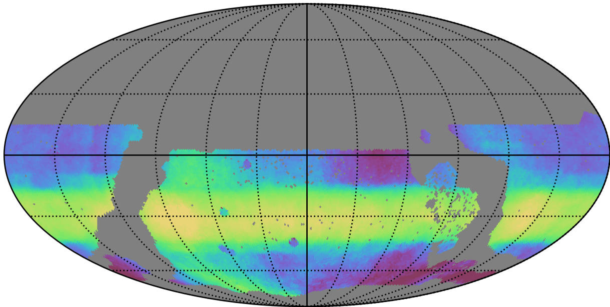
too_elab_r8_d2_griz_v3.4_10yrs WFD all bands: Median HA
