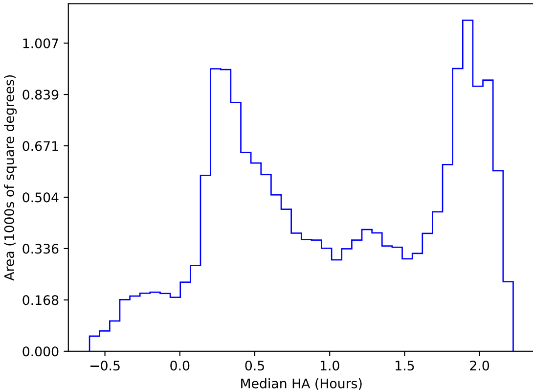
too_elab_r8_d2_griz_v3.4_10yrs WFD all bands: Median HA
