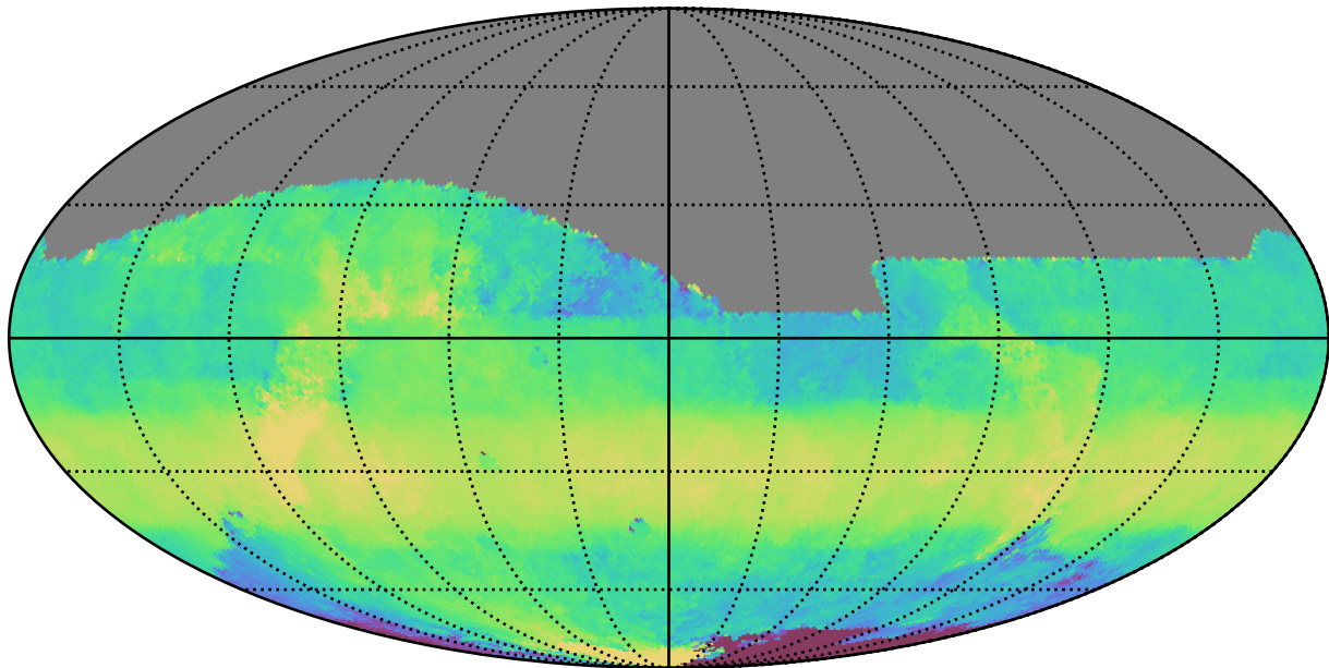
too_elab_r8_d2_griz_v3.4_10yrs All sky z band: Median HA
