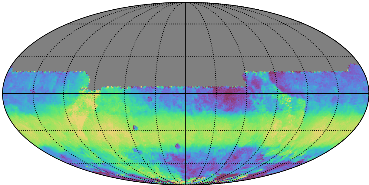
too_elab_r8_d2_griz_v3.4_10yrs All sky y band: Median HA
