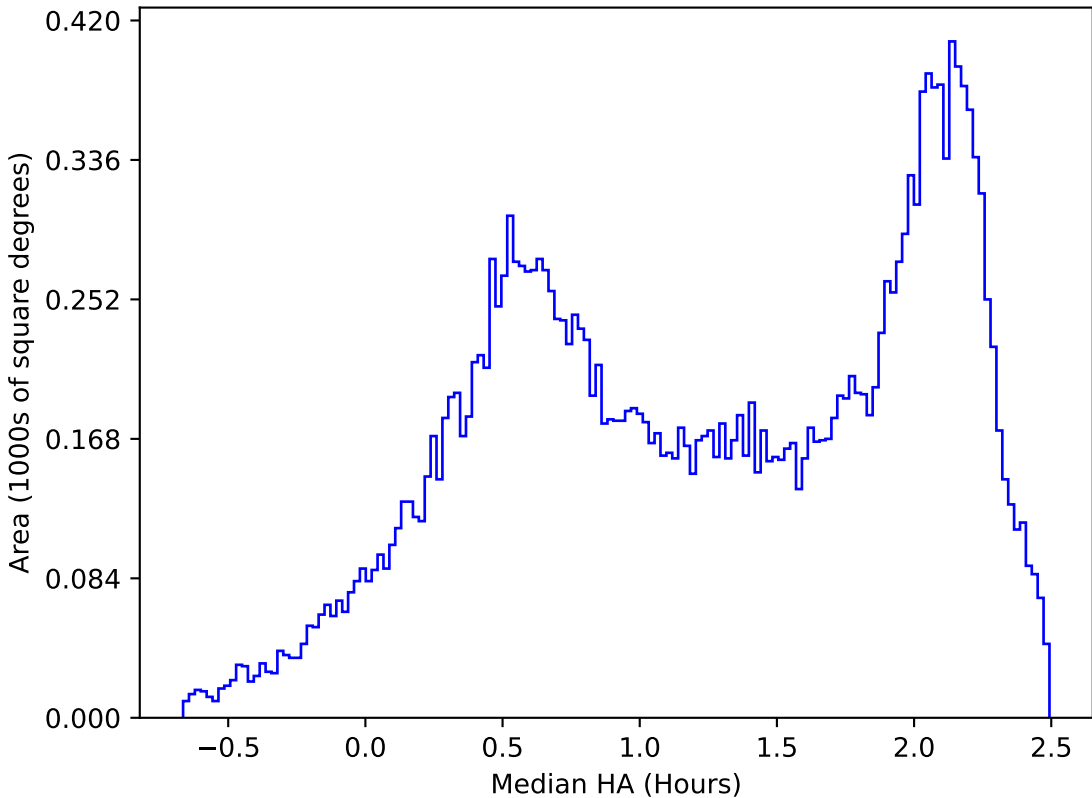
too_elab_r8_d2_griz_v3.4_10yrs All sky y band: Median HA
