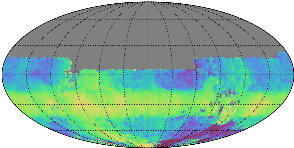
too_elab_r8_d2_griz_v3.4_10yrs All sky u band: Median HA
