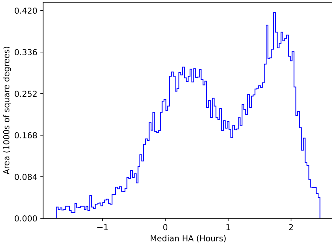
too_elab_r8_d2_griz_v3.4_10yrs All sky u band: Median HA
