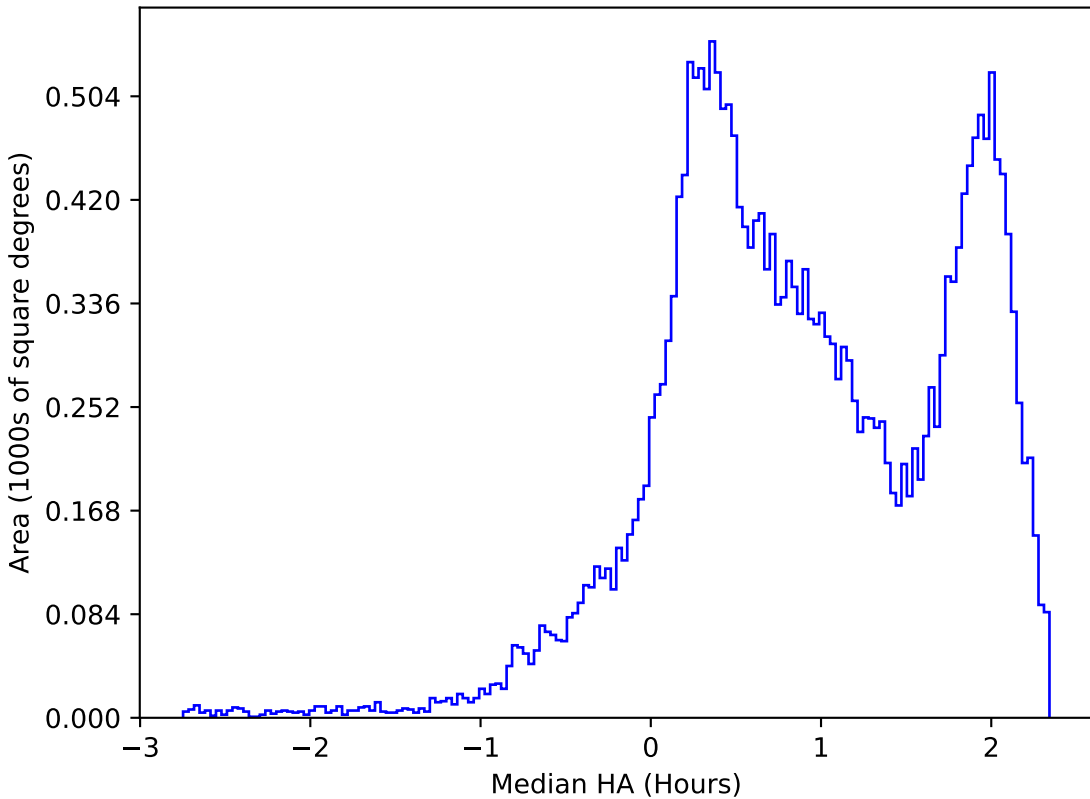
too_elab_r8_d2_griz_v3.4_10yrs All sky i band: Median HA
