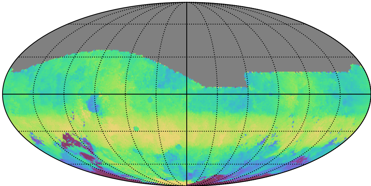
too_elab_r8_d2_griz_v3.4_10yrs All sky g band: Median HA
