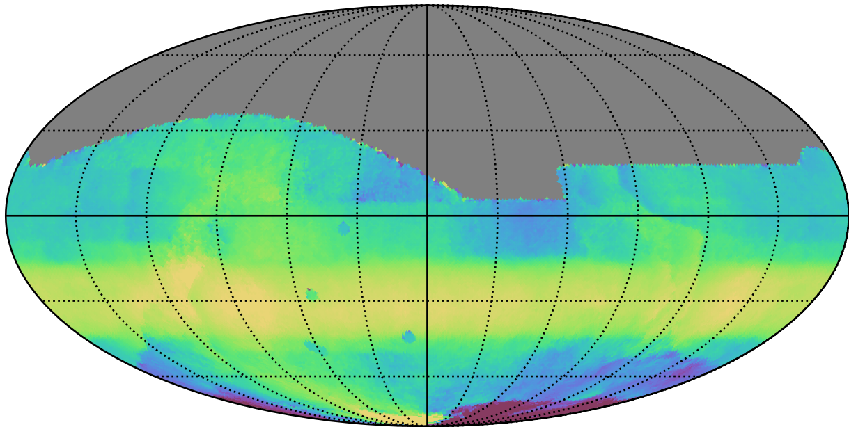
too_elab_r8_d2_griz_v3.4_10yrs All sky all bands: Median HA
