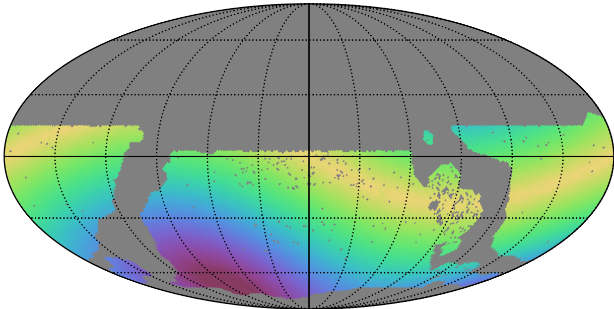
too_elab_r8_d2_griz_v3.4_10yrs WFD z band: Max solarElong
