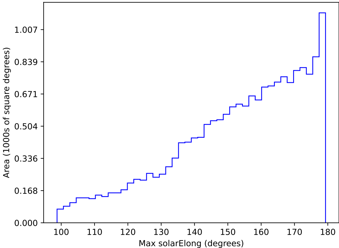
too_elab_r8_d2_griz_v3.4_10yrs WFD z band: Max solarElong
